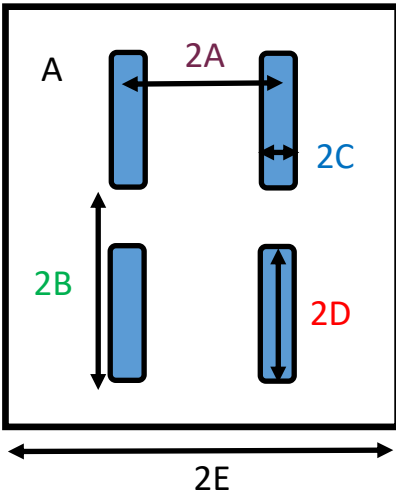
Dual Slot
