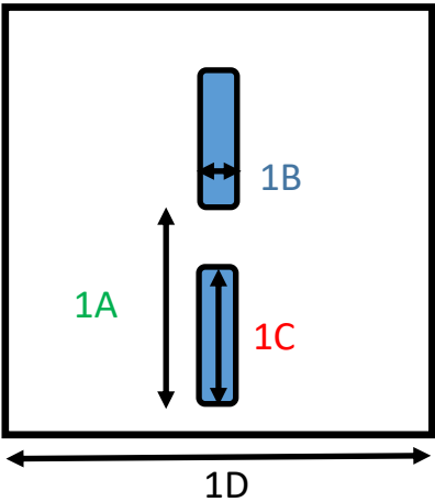
Single Slot
